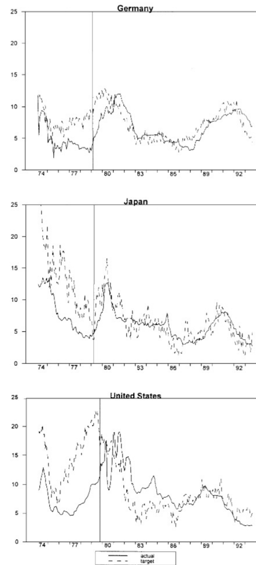
Fig. 2. G3 interest rates: target vs. actual.
